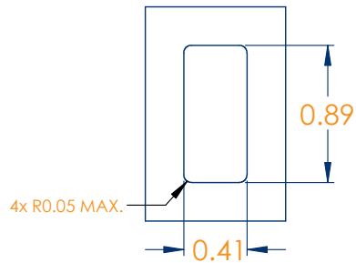
PANEL CUTOUT DIMENSIONS (PANEL THICKNESS UP TO 0.125")
