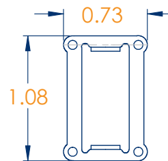
PANEL CUTOUT DIMENSIONS (PANEL THICKNESS UP TO 0.125")
