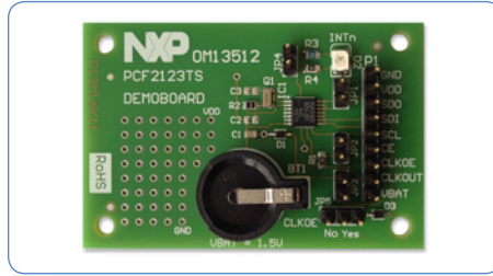
OM13512 PCF2123 SPI-bus RTC demo board
